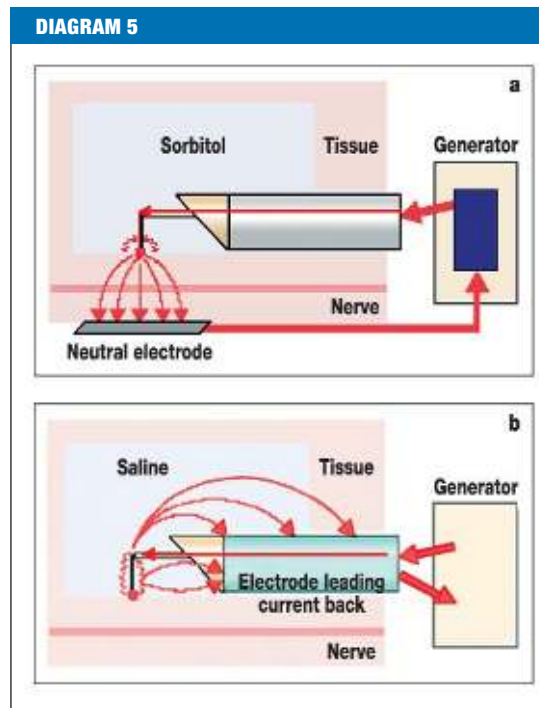
Resection mechanism in a) classic (monopolar) resection. The resistance of the sorbitol is greater than that of the tissue. b) In bipolar resection, no current flows into the tissue because the tissue's resistance is greater than that of the saline.
